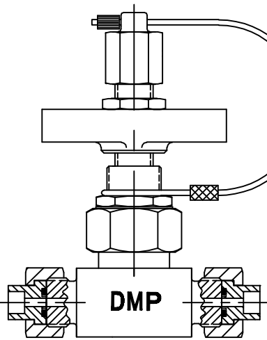
UNION ENDS SERIES M1156
