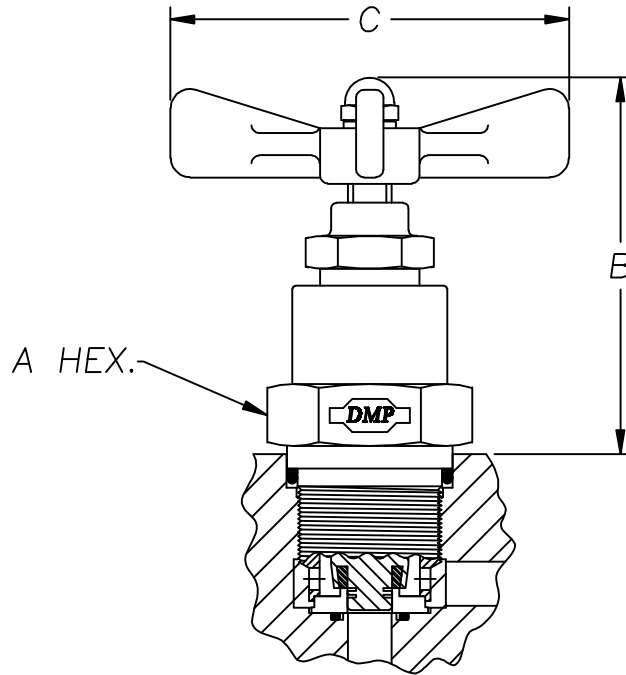
SHUTOFF VALVE CARTRIDGE CAT NO. M236
