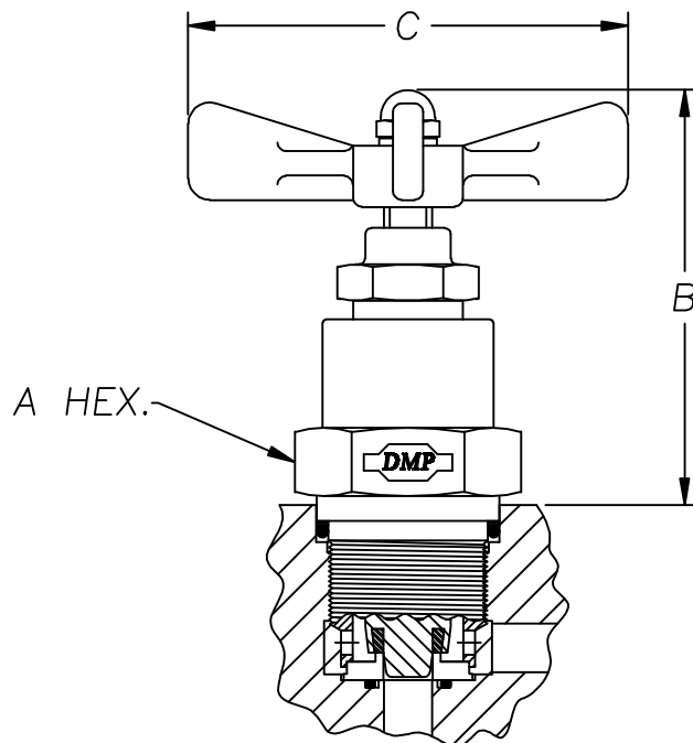
NEEDLE VALVE CARTRIDGE CAT NO. M246
