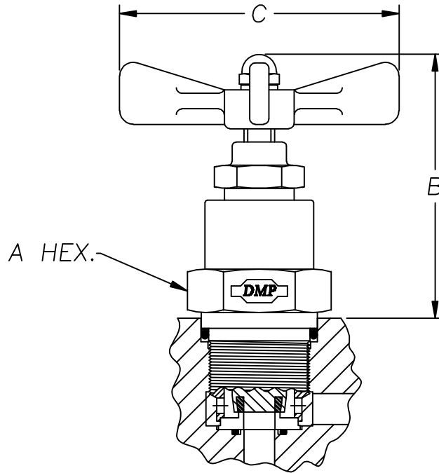
STOP CHECK VALVE CARTRIDGE CAT NO. M256
