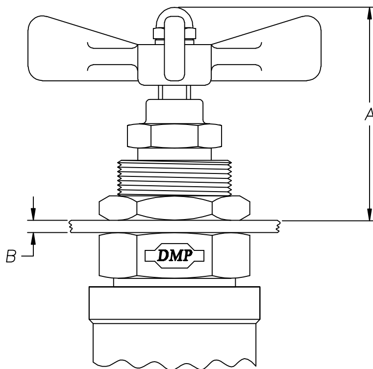
PANEL MOUNTING DIMENSIONS
