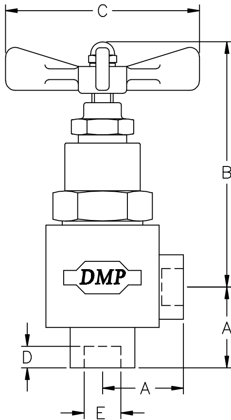
ANGLE GLOBE SHUTOFF VALVE DIRECT WELD CAT NO. M7136
