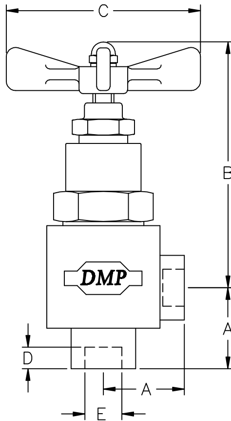
ANGLE GLOBE NEEDLE VALVE DIRECT WELD CAT NO. M7146
