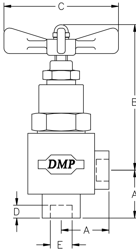
ANGLE GLOBE STOPCHECK VALVE DIRECT WELD CAT NO. M7156
